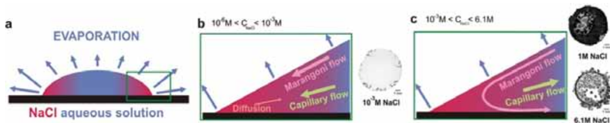
Figure 1: (a) Evaporation behavior of a sessile droplet from aqueous sodium chloride solutions. Locally varying evaporation rate and resulting concentration gradient: below (b) or above (c) 10^{-3}\text{M} NaCl. Typical microscopy images of the final deposit patterns from droplets of 10^{-3} and 6.1M NaCl on silica wafers at T = 25^\circ\text{C} and \text{RH} = 0\% .
