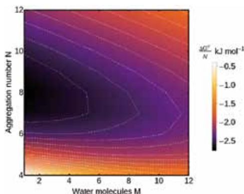
Figure 1: Calculated standard Gibbs energy \Delta G^\circ potential surface.
