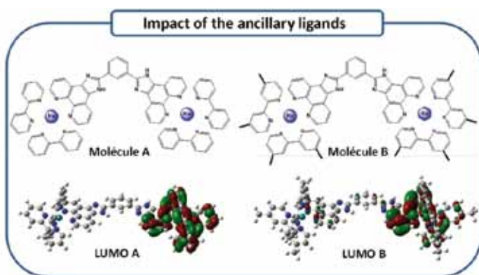
Figure 1: Studied DIP ligands, CO 2 photoreduction and related TD-DFT calculation.
