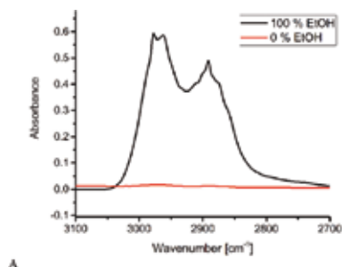
Figure 2 (left side): principle of operation of the on-line measurement of solvent activity by IR adsorption (middle): Absorbance signal obtained for 100% ethanol and 0% ethanol (right: values obtained for the ethanol activity in the vapour phase in equilibrium with ethanol/water mixtures: comparison of the values measured and obtained by head-space chromatography. Note that these values can also be obtained via molecular dynamics 8 .
