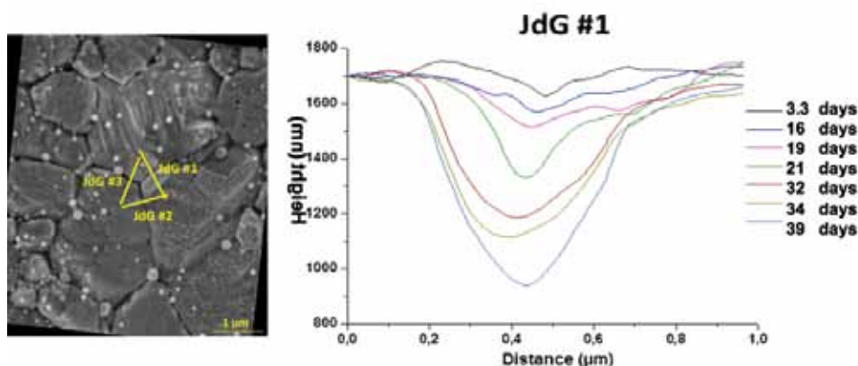
Fig. 1. Evolution of the height profiles perpendicular to a grain boundary obtained during the dissolution of sintered pellet of \text{UO}_2 + 3 mol% PGM in 0.1 mol.L -1 \text{HNO}_3 at 60 °C.
