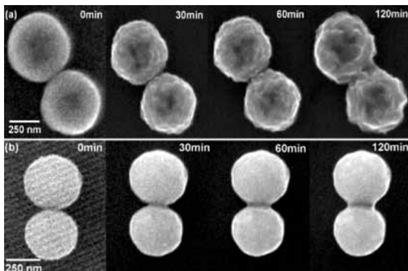
Fig. 1. In situ HT-ESEM observation of \text{CeO}_2 microspheres sintering at 1050°C: (a) poly- and (b) single-crystal particles 2 .
