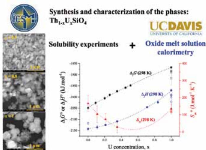
Fig. 1: Determination of thermodynamic properties of uranotorite solid-solutions combining wet chemistry route of synthesis, solubility experiments and calorimetry.
