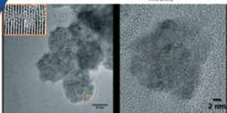
Growth of UO_2 microspheres
