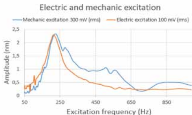
Figure 4: Reciprocity of Onsager coefficients: the same bubble is excited either with electrical excitation produced by the electrodes, or by mechanic excitation via a piezo-electric device located in the bottom of the cell. The main excited mode is the same, but other modes are excited also by echo of the sound on the sample reservoir. Measurement of the hydrostatic pressure and the electrical field of same frequency responsible of the same surface wave amplitude would provide unique information about the energy needed to produce the waves, and therefore the first direct verification (and exploitation) of Onsager reciprocity principle.
