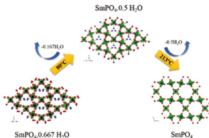
Figure 1. Dehydration scheme of the \text{SmPO}_4 \cdot 0.667 \text{H}_2\text{O}
