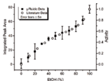
Figure 2 (left side): principle of operation of the on-line measurement of solvent activity by IR adsorption (middle): Absorbance signal obtained for 100% ethanol and 0% ethanol (right: values obtained for the ethanol activity in the vapour phase in equilibrium with ethanol/water mixtures: comparison of the values measured and obtained by head-space chromatography. Note that these values can also be obtained via molecular dynamics 8 .
