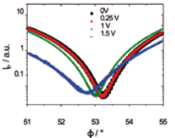
Fig. 1: Ellipsometry set up with a newly designed US cell (top). Reflectivity measurements at the water/air interfaces (down) at different US intensities (in volt). The shift in the minimum Intensity I_p has been attributed to a macroscopic interface deformation induced by US. For low US intensity (0.25 V) the surface roughness is in the nanometric range.
