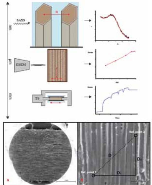
Figure 1: swelling of wood in osmotic equilibrium with atmosphere of a solution of electrolytes is investigated by Small angle X-ray micro-diffraction at the nanometre scale (top), via environmental scanning electron microscopy (middle) at the micron scale as shown below so lateral and longitudinal swelling can be obtained independently and finally at macroscopic scale using a tensile stage (bottom).
