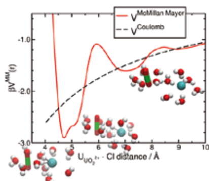
Figure 1: \text{UO}_2^{2+} - \text{Cl}^- McMillan-Mayer potential profile. Characteristic snapshots of hydrated \text{UO}_2\text{Cl}^+ complexes are also shown. Uranium is in green, chloride in cyan, oxygen atoms in red, and hydrogen atoms in white.
