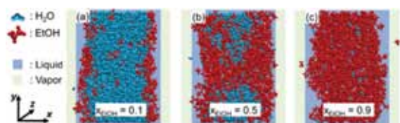
Figure 3: Snapshots representing the liquid phase in contact with vapor phases for different ethanol mole fractions.
