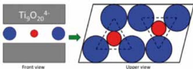
Figure 2: Representation of triangular geometry of the sodium hydrate in porous media, the blue and red spheres are water molecules and sodium ions, respectively.
