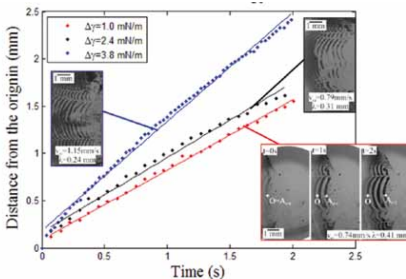
Figure 2 : Distance from the origin evolution in time during fringes formation at different surface tension gradient \Delta\gamma . The oxalic excess (0,6M) and the average contact angle ( \theta_a=9+0.5^\circ ) are identical for all experiments. The Marangoni flow speed, v_M , increases with the surface tension gradient whereas the wavelength of the periodic pattern, \lambda_c , decreases.
