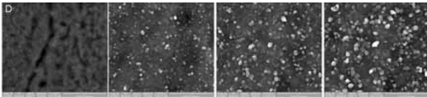
Fig. 2. Image series showing the formation of \text{MnCr}_2\text{O}_4 spinel crystals during the oxidation of a Ni-30Cr + 1.5wt%Mn alloy at T=1000^\circ\text{C} , P_{\text{atm}}=200\text{Pa} .
