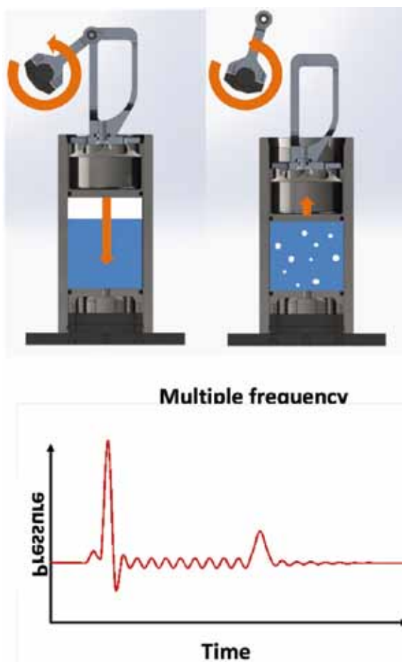
Fig.1: Schematic representation of the shock induced reactor and the generated pressure wave within the liquid.
