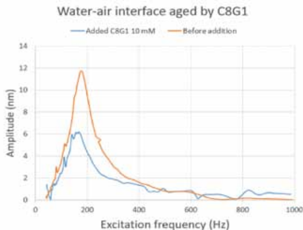
Figure 3: Sensitivity to the presence of a common protein membrane solubilizer (octylglucoside) on the surface of a bubble: one molecule per \text{nm}^2 induces a downshift of the resonance with an increase of relaxation producing FWHM broadening from Q = 0.6 to Q' = 0.75 (10 mM C8G1); curve in orange : no octylglucoside, and in blue : with octylglucoside.
