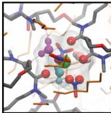
Figure 1: Snapshot obtained from MD simulations representing an aggregate of \text{La}(\text{NO}_3)_3 \cdot 4(\text{H}_2\text{O})_3 in n -heptane with colored water molecules: WAT0 (pink), WAT1 (cyan), and WAT2 (purple) where the number after WAT corresponds to the number of DMDOHEMA molecules H-bonded to the water molecule. For the illustration, \text{La}^{3+} is colored in green, oxygen atoms are in red, nitrogen atoms are in blue, carbon atoms are in black, and hydrogen atoms are in white. n -Heptane molecules are colored in orange.
