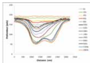
Fig. 2. a) Image series recorded during the dissolution of a \text{Ce}_{0.2}\text{Nd}_{0.8}\text{O}_2 ceramic in HCl 0.1M for 1200s. c) Height profile series extracted from the image series along the orange line drawn in the picture '1200s'.
