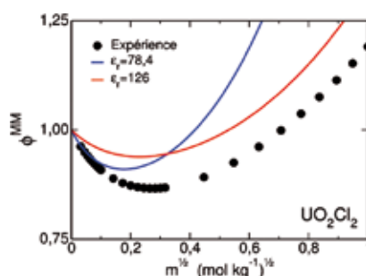
Figure 2: Osmotic coefficients in the McMillan-Mayer frame of reference for \text{UO}_2\text{Cl}_2 obtained experimentally (circles) and from coarse-grained atomistic simulations (lines) as a function of the square root of the concentration.
