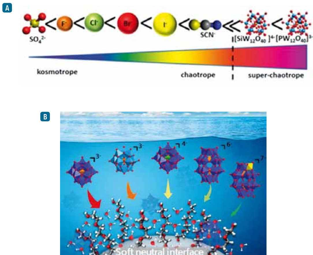
Fig. A Beyond the Hofmeister series on the "chaotropes" side with Kegging POM as an example. B Schematic representation of various POM anions in interaction with non-ionic micelles, the strength of the interaction depends on the POM's charge density decrease from right to left.
