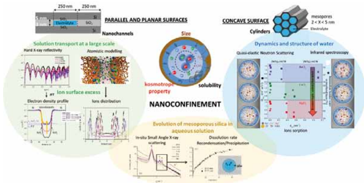
Figure 1: Scientific approach used to study the physical and chemical properties of nanoconfined water in presence of ions.
