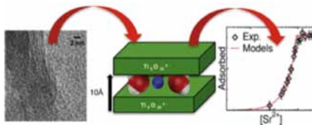
Figure 1: Combined experimental and mesoscopic modeling approaches used for the sodium nanotitanate.
